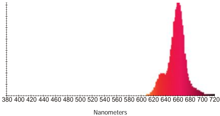
Spectral Energy Distribution
