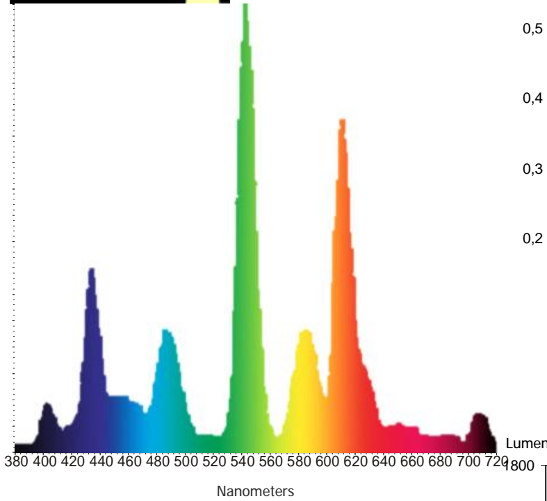
Discharge With Low Pressure Mercury Vapor
