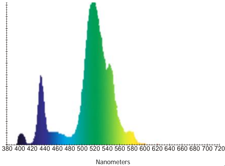
Discharge With Low Pressure Mercury Vapor
