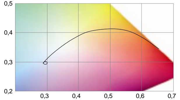
CIE 1931 Coordinates
