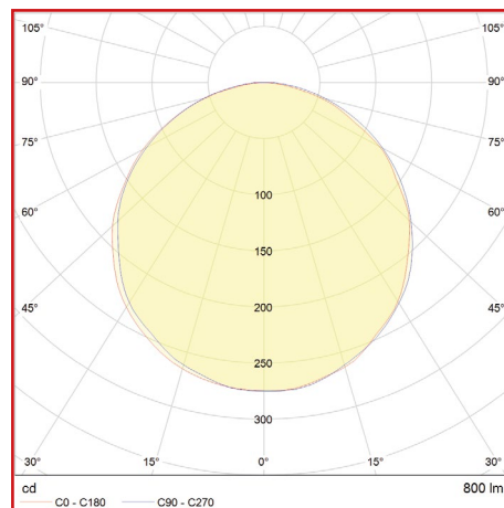
Low Power - 4000K - Clear Diffuser
