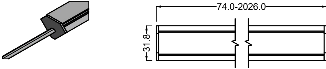
Standard Cable Entry 300mm Tail
