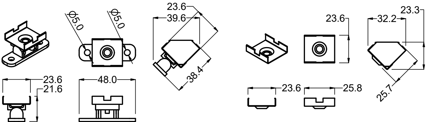
Adjustable Bracket
