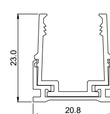
Hybrid Aluminium & Clear Plastic Profile
