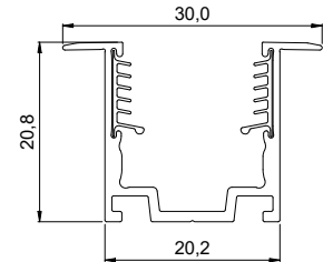
Serrated Recessed Aluminium Profile
