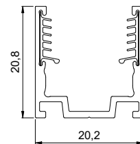
Serrated Aluminium Profile
