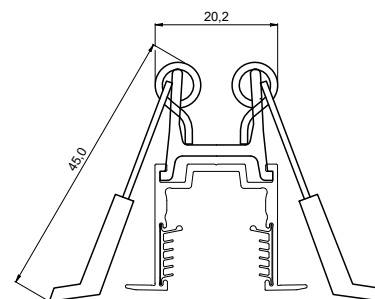
Ceiling Mounting Clip (to be supplied with Serrated Recessed Mounting Profile)
