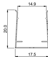
Flexible S/S Profile
