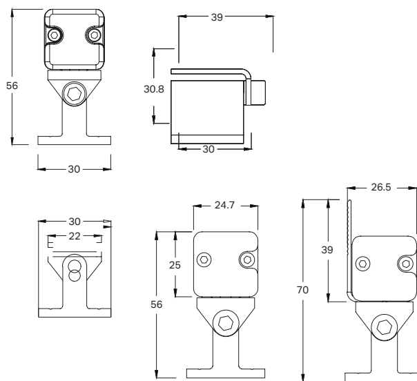
Adjustable Bracket A1
