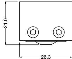
PROFILE WITH FIXED BRACKET
