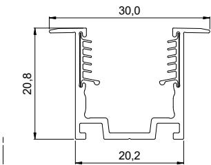
Flanged Serrated Aluminium Profile
