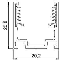
Bendable / Serrated Aluminium Profile
