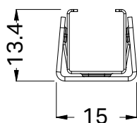
MOUNTING CLIP - FX9001
