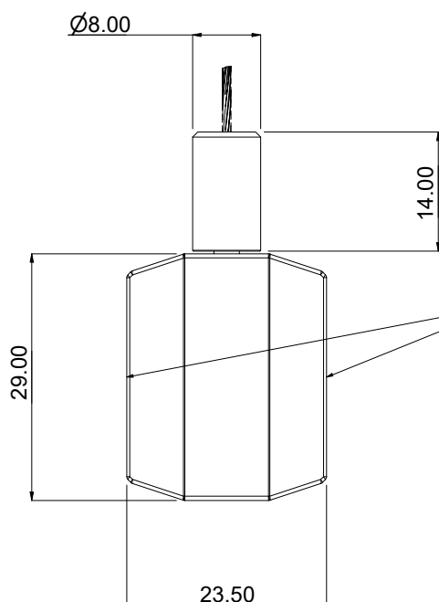
SECTION DETAIL
