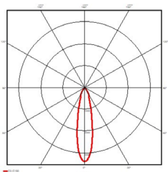
17° Beam Angle
