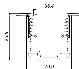
Flanged Serrated Aluminium Profile
