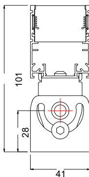
Adjustable bracket with 36mm and 50mm Aluminium profile
