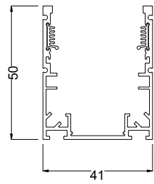
50mm Aluminium profile (inc cable void)
