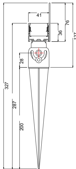
Ground spike adjustable bracket
