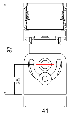
Adjustable bracket with 36mm and 50mm Aluminium profile
