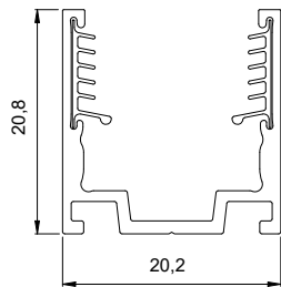
Bendable / Serrated Aluminium Profile
