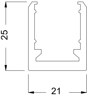
Silicone Flexible Profile
