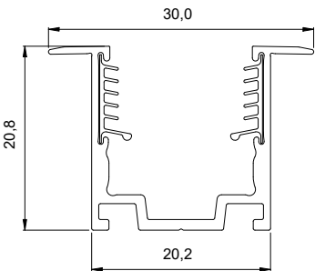
Flanged Serrated Aluminium Profile
