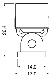
PROFILE WITH ADJUSTABLE BRACKET
