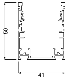
50mm Aluminium profile (inc cable void)
