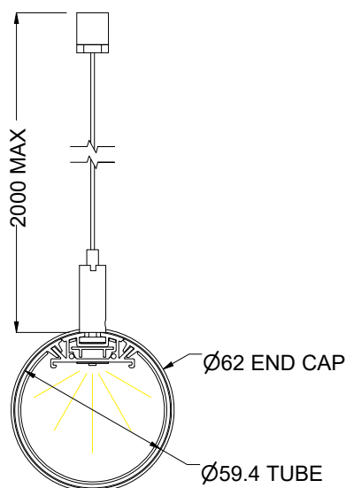
Suspended Mounting
