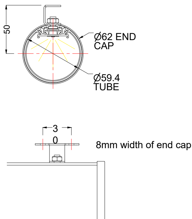
Surface Mounting
